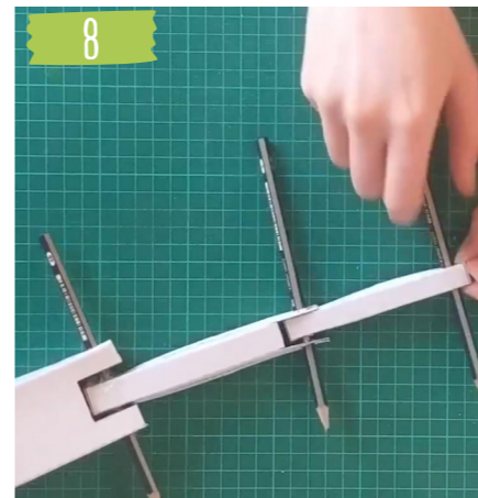
Assemble part 2 and three together using another pencil. Then add the 3rd pencil to the end of part 3.
